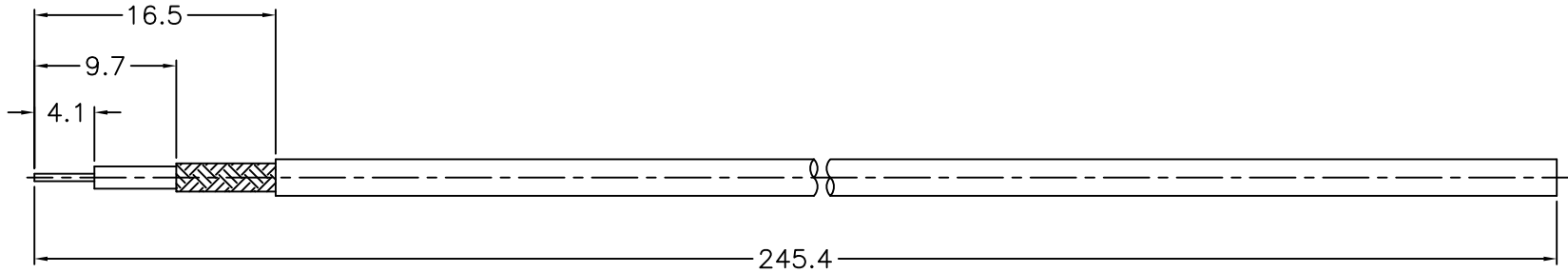
RECOMMENDED CABLE STRIPPING DIM'S (建議剝線尺寸)
