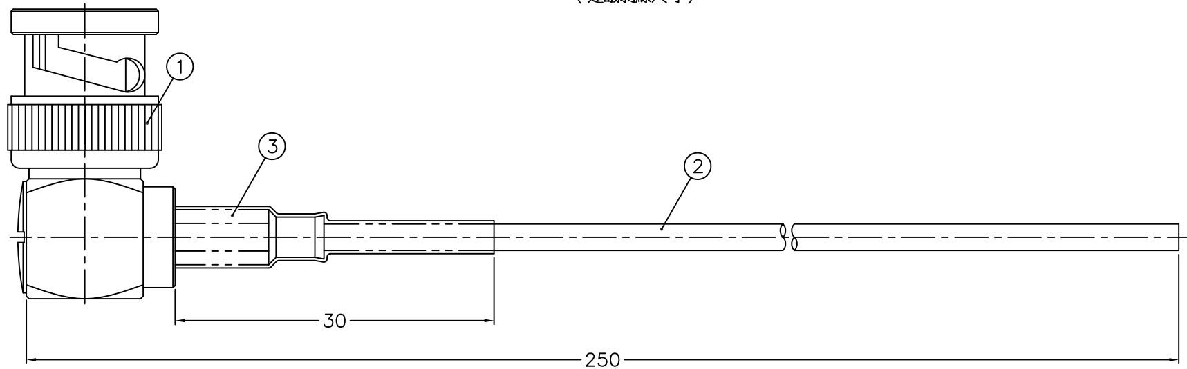
RECOMMENDED CABLE STRIPPING DIM'S (建議剝線尺寸)
