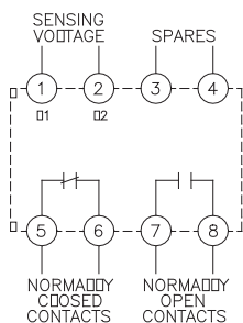
Single Phase
